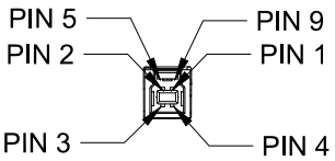
9-PIN FEMALE USB-B MATING FACE
